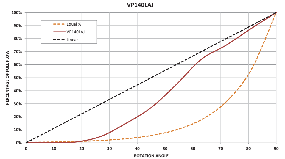
Figure 7: VP140Lxx and VP140Mxx flow rate charts
